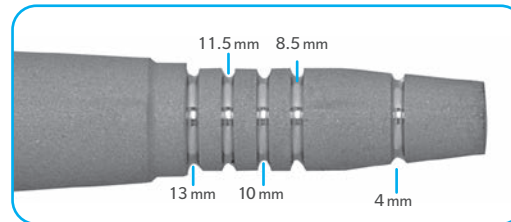
Operating end of the Osteotome
